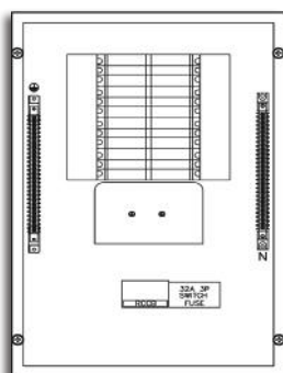
SWITCH INCOMER
