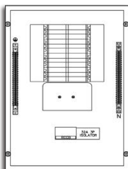
ISOLATOR INCOMER
